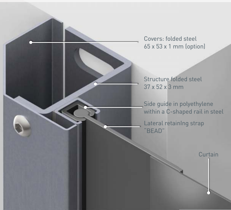
Low friction side guide
